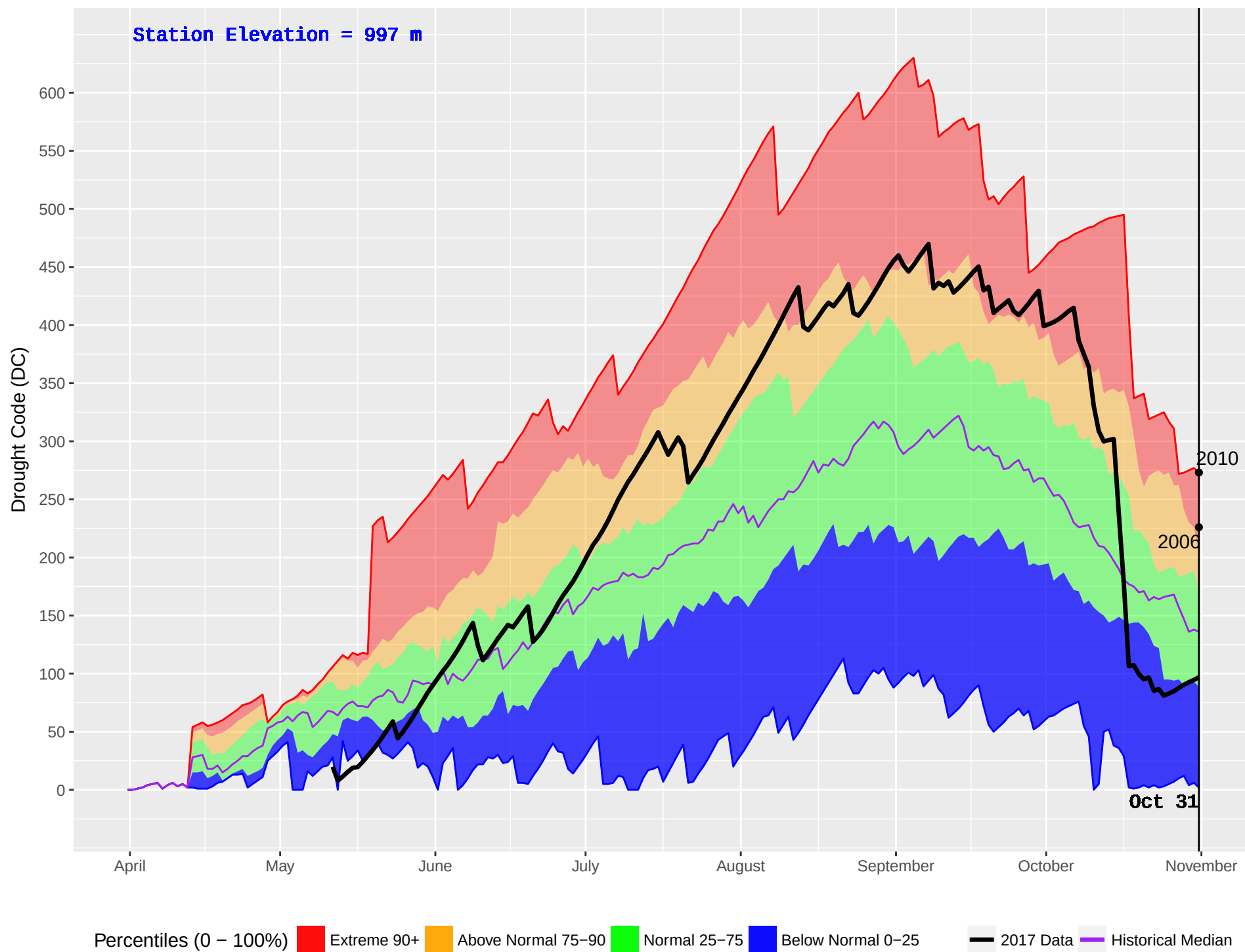
JERRY (190) : Historical (1988–2016) and Current (2017) Noon Drought Code (DC)
