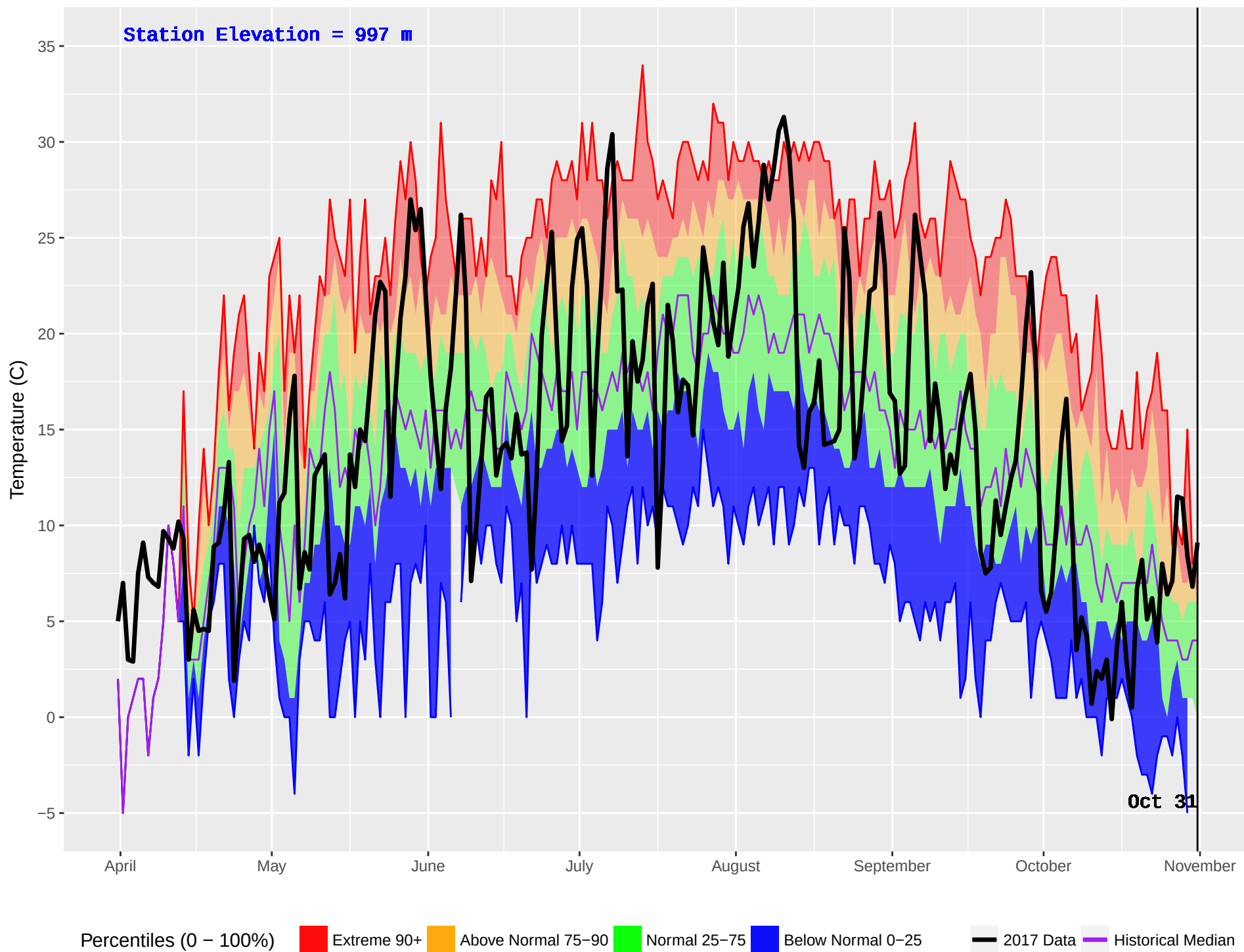
JERRY (190) : Historical (1988–2016) and Current (2017) Noon Temperature
