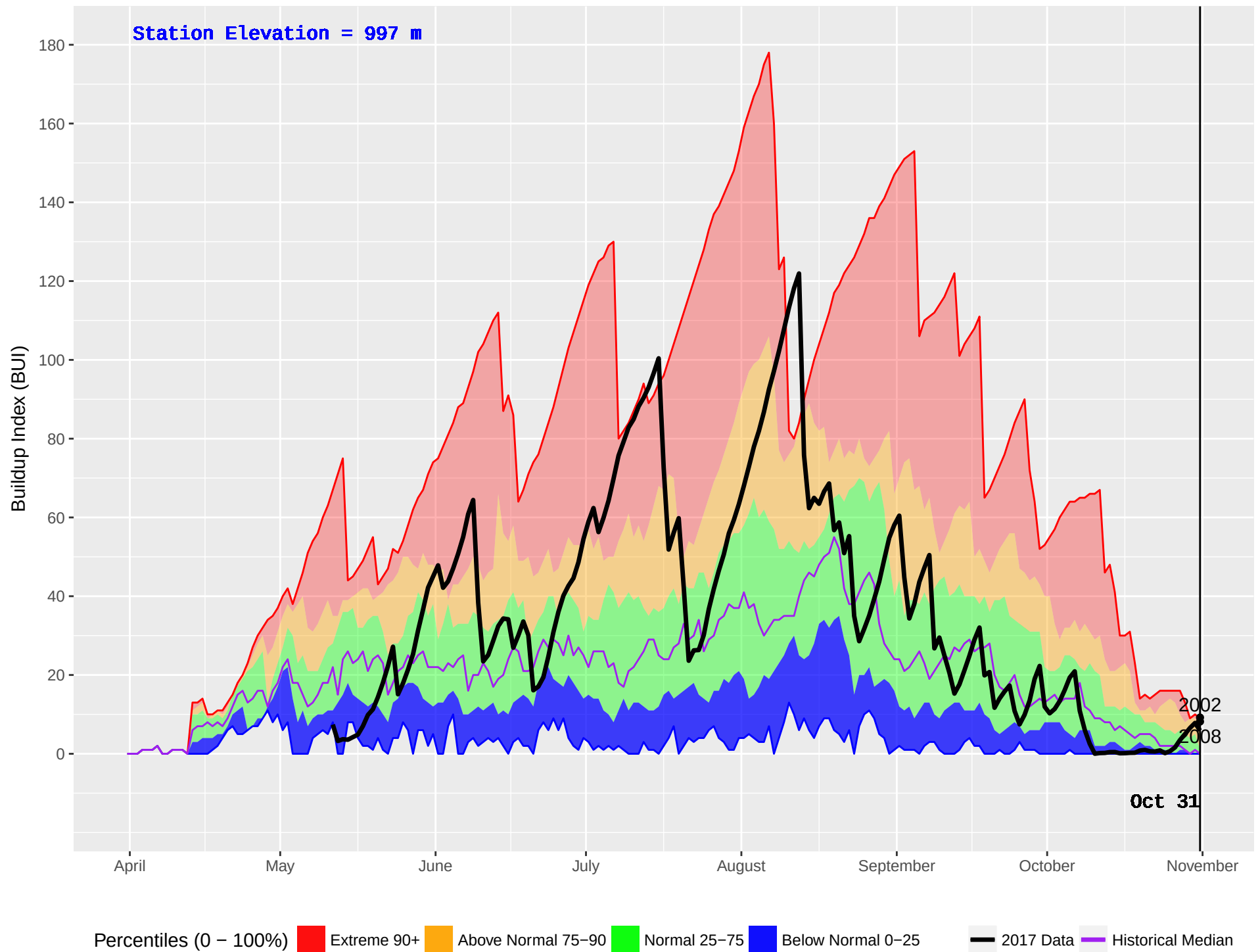
JERRY (190) : Historical (1988–2016) and Current (2017) Noon Buildup Index (BUI)
